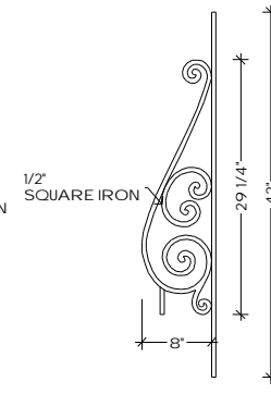
TOP VIEW B-1 FLAT
