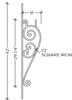
TOP VIEW B-3 ALL RADIUS FROM 28" TO 20'-0"
