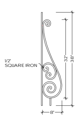
TOP VIEW A-3 ALL RADIUS FROM 28" TO 20'-0"
