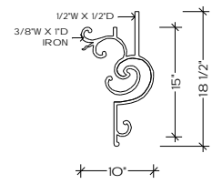
TOP VIEW C-1 FLAT
