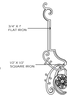
RIGHT SIDE TERMINATION LEFT SIDE VIEW
