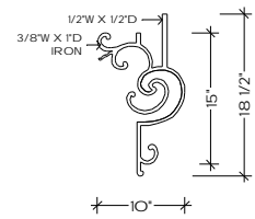
TOP VIEW C-2 ALL RADIUS FROM 30" TO 20'-0"
