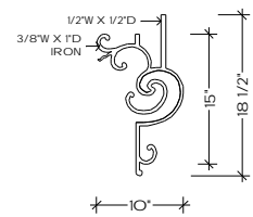
TOP VIEW C-3 ALL RADIUS FROM 30" TO 20'-0"
