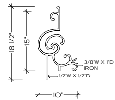
TOP VIEW C-3 ALL RADIUS FROM 30" TO 20'-0"
