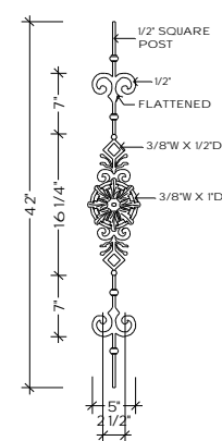
TOP VIEW FLAT
