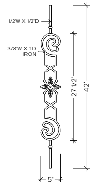
PIECE D FITS ALL ANGLES & LEVEL BALCONY
